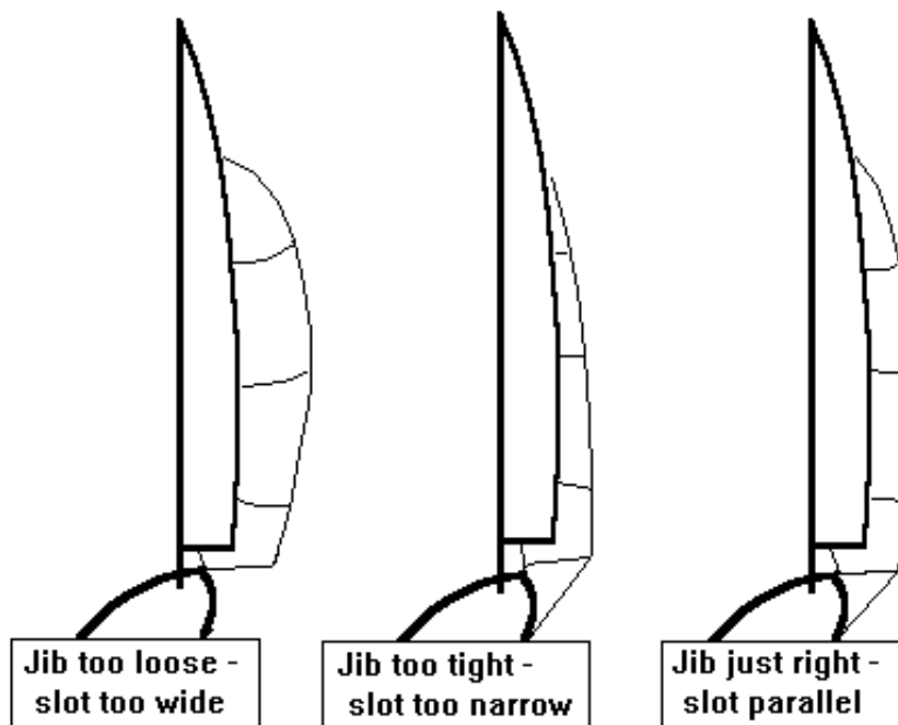
View of jib/main "slot" from behind boat
